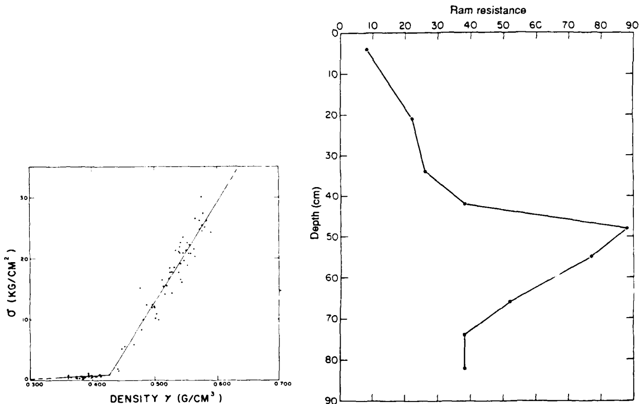
Figure VI-3. Uniaxial compressive strength of natural South Pole snow plotted against bulk density (test temperature -50^{\circ}\text{C} ) (Ramseier 1963).
